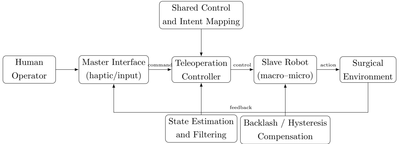
Figure 6: Simplified teleoperation architecture for macro–micro surgical robotics. The reviewed literature addresses different parts of this loop, including state estimation, shared control, predictive control, and transmission compensation.
